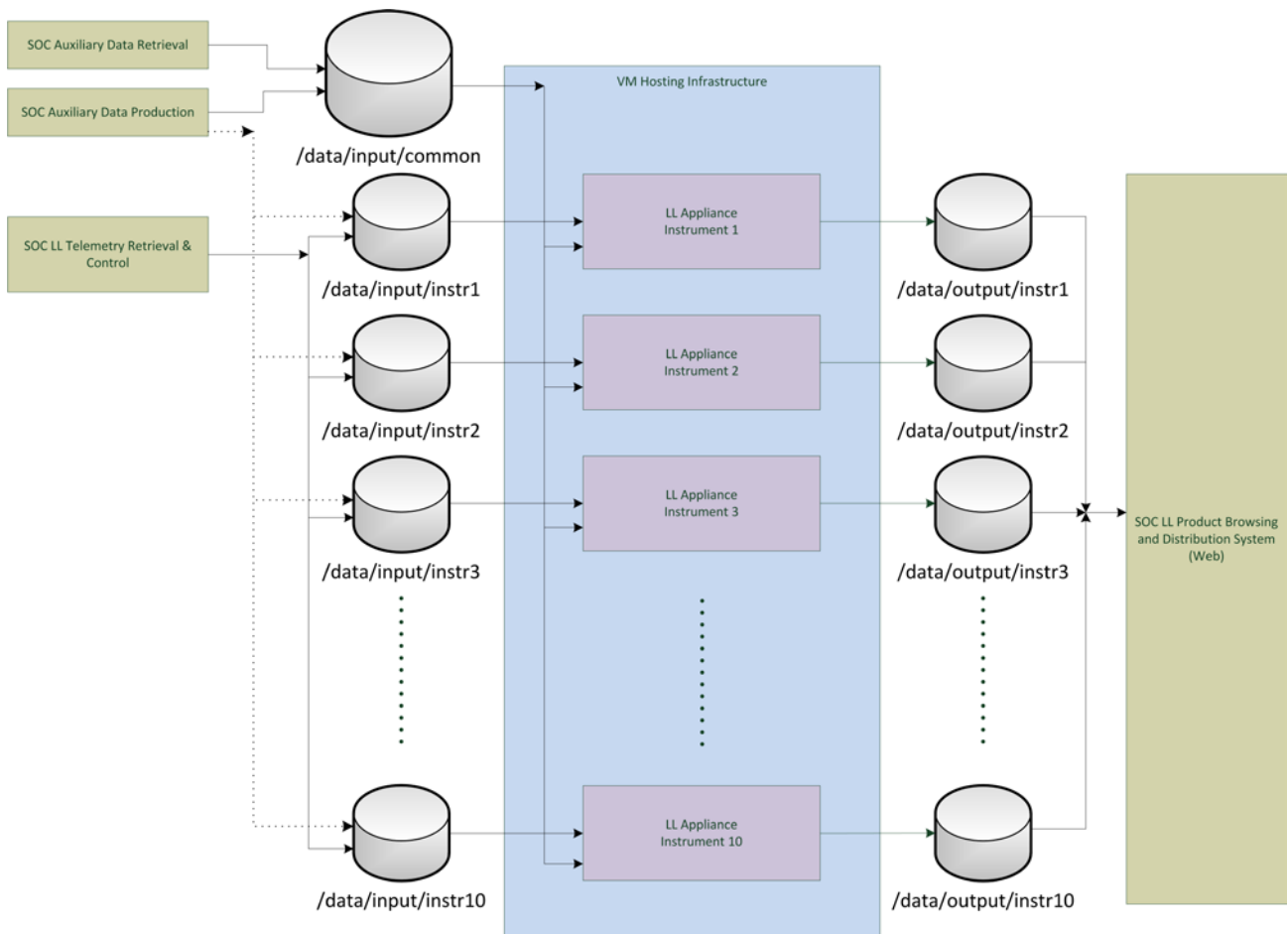
Figure 2 SOC Low-Latency Appliance Deployment Context
